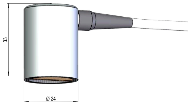
Housing DSE 18
