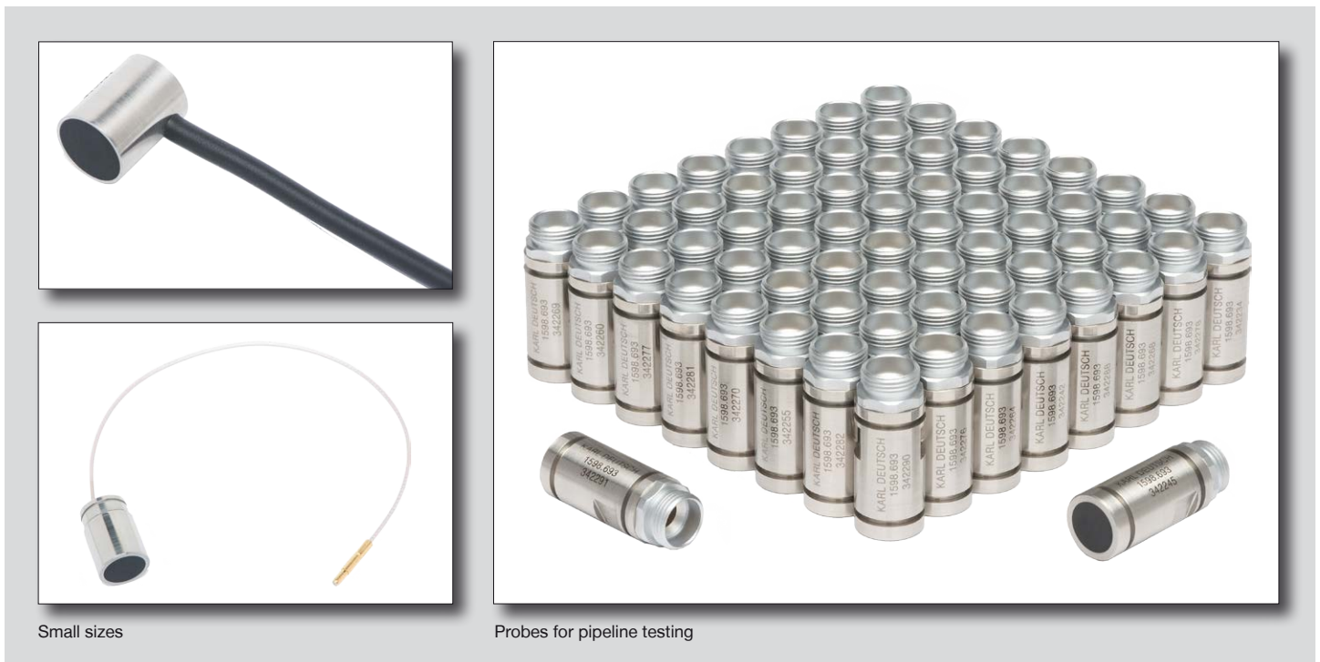
Immersion probes for automated testing (hermetic) Various designs (line or point focused, angle probes, T/R probes) Connection technique (cables, connectors)
